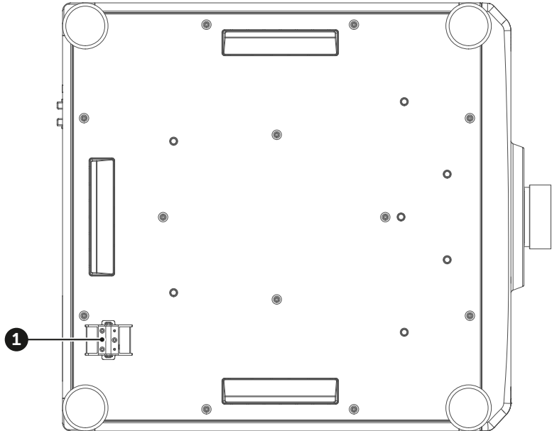
Image 2-4 Bottom view
